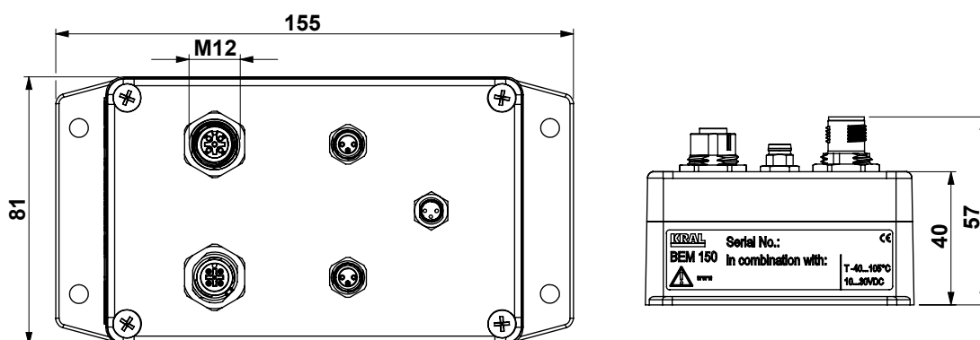
Fig. 2: Dimensional drawing processing unit
