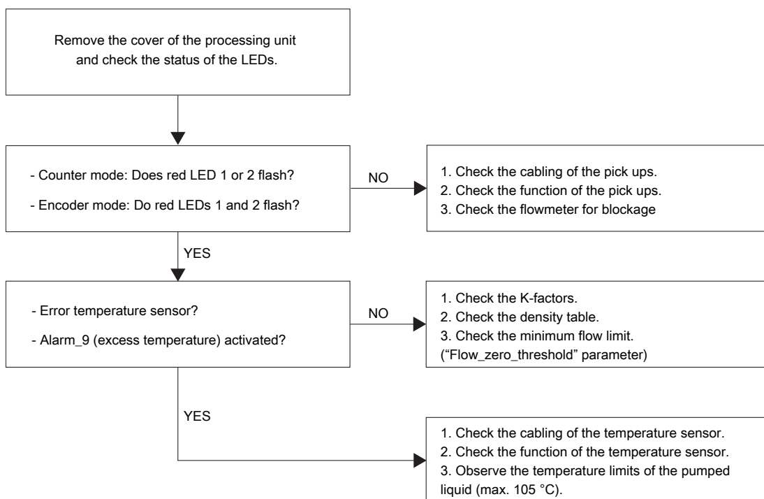
Fig. 12: Error tree: No flow
