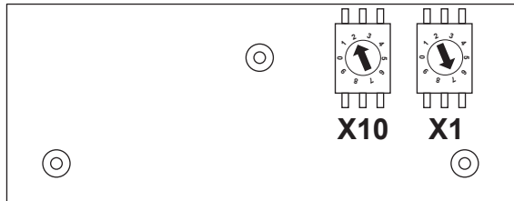
Fig. 8: Modbus addressing
