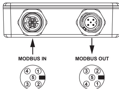
Fig. 5: Pin assignment
