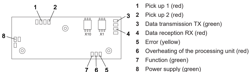
Fig. 9: Status LEDs
