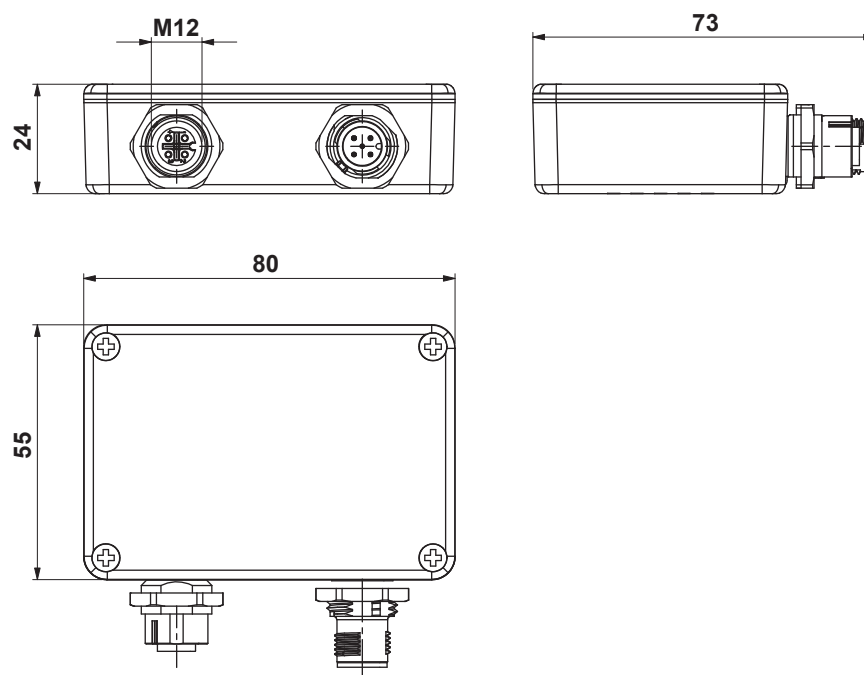
Fig. 2: Dimensional drawing processing unit
