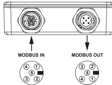
Fig. 3: Pin assignment
