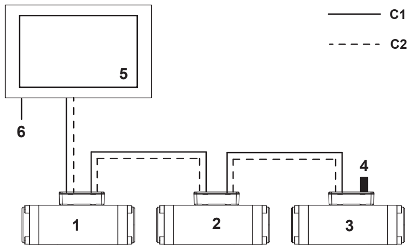
Fig. 4: Connecting several processing units
