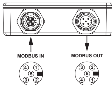
Fig. 3: Pin assignment
