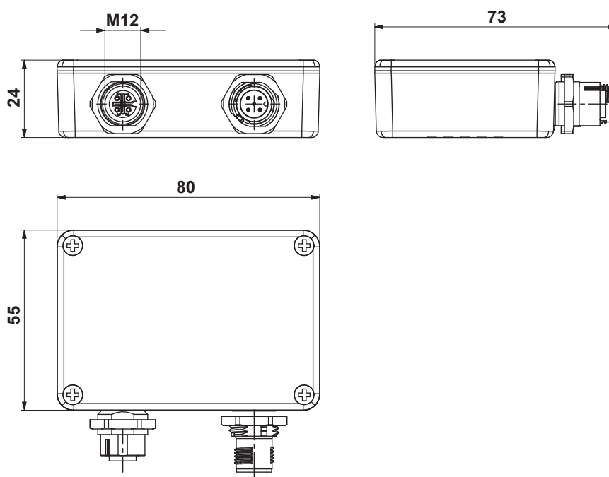
Fig. 2: Dimensional drawing processing unit
