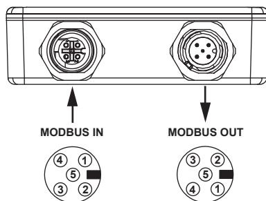
Fig. 5: Pin assignment
